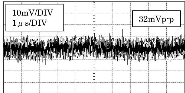
5V, C14
