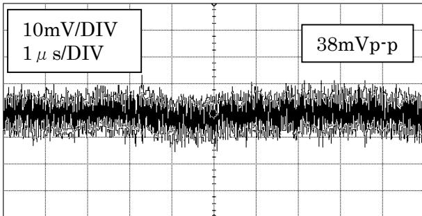
5V, C12
